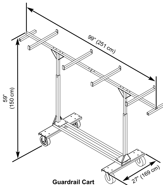
Guardrail Cart
