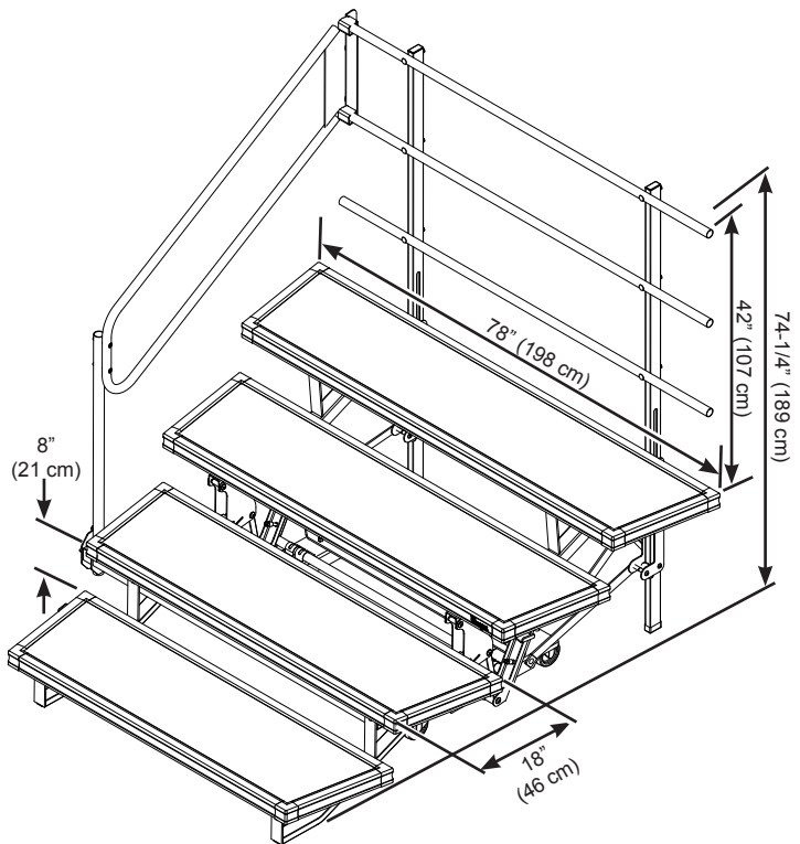
4-Step Riser with Optional Side Rail
