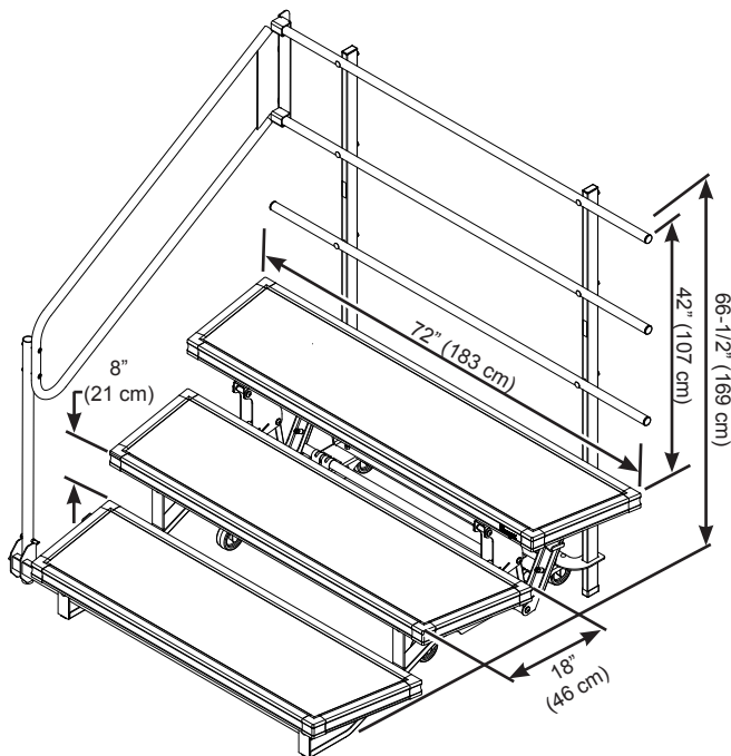
3-Step Riser with Optional Side Rail
